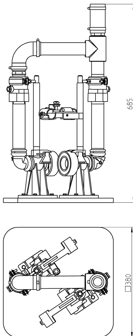
Dimensions Easyfix 32 Duo (mm)
