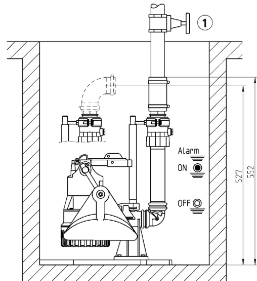
Dimensions and switching points speical float (mm)
