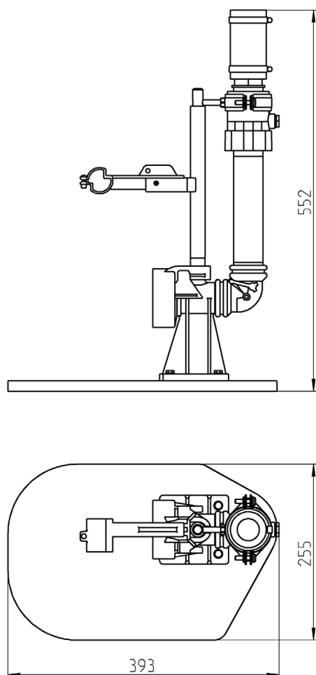
Dimensions Easyfix 32 Single (mm)
