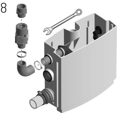
- Install the pressure outlet
